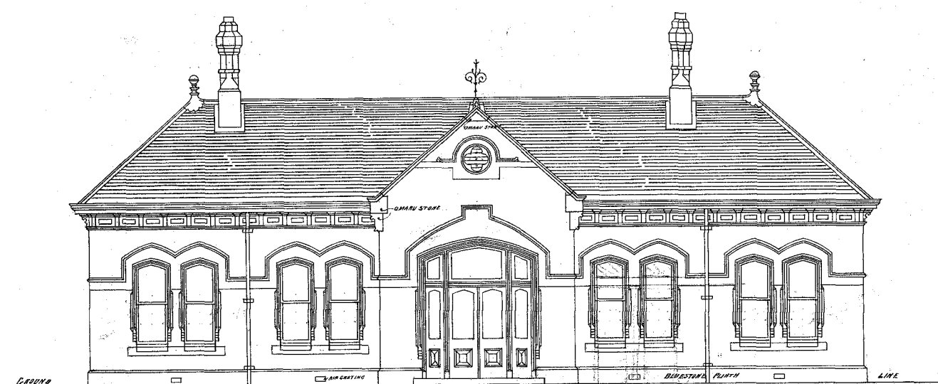
ELEVATION TOWARDS ROAD
