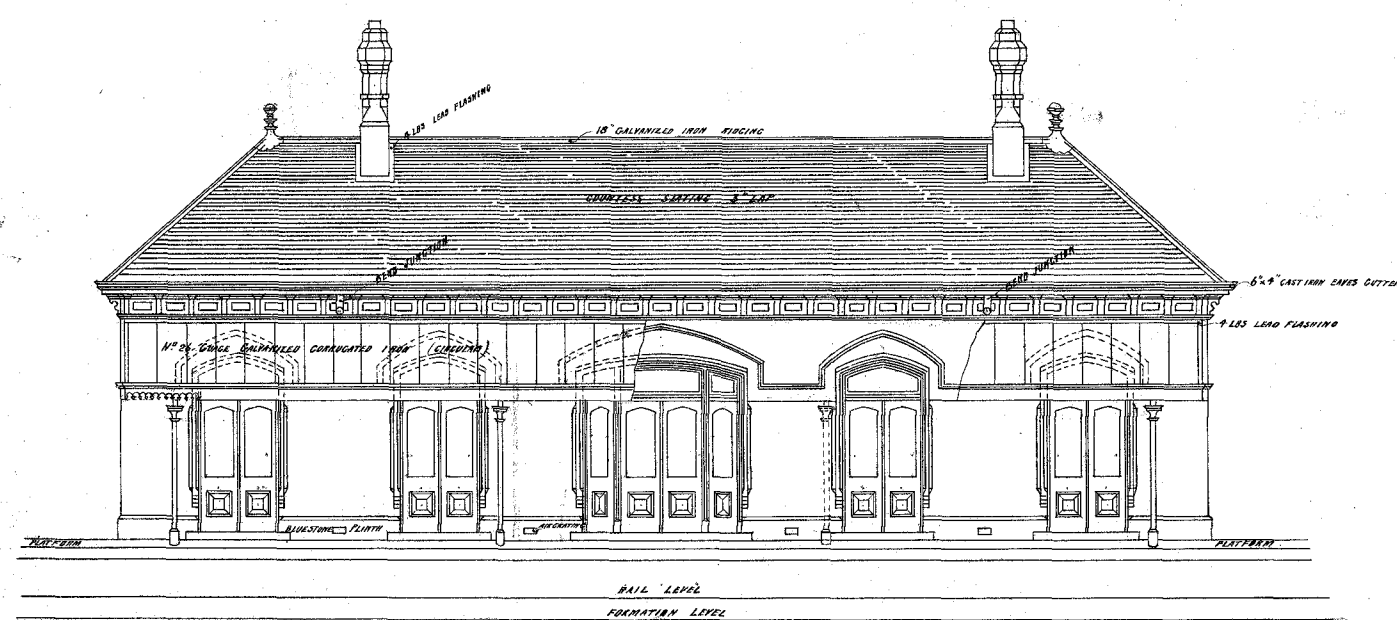
ELEVATION TOWARDS PLATFORM
