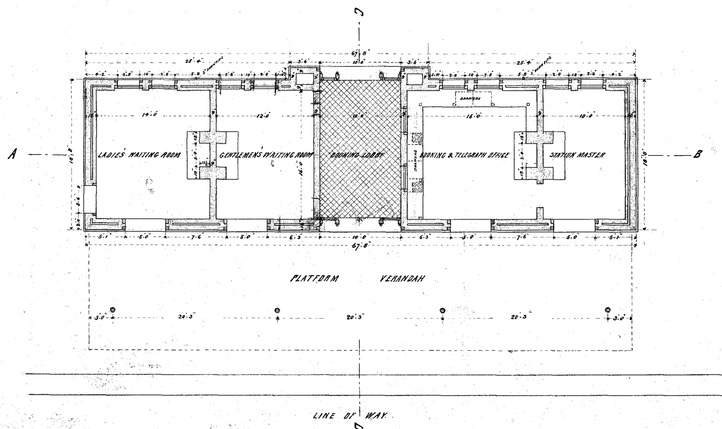
GROUND PLAN
