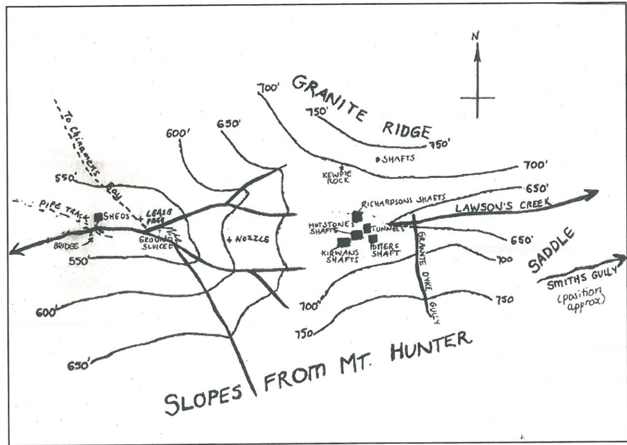
Figure 1: Sketch map of major Mt Hunter Tin Mine shafts at Lawson's Creek, drawn by William Ferguson, geological surveyor, in June 1925. Source: McKellar, I.C. 1993. The Rise and Fall of the Mt Hunter Tin Mine . I. & M. McKellar: Heathmont. Page 26.
